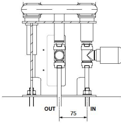
Detail connection
